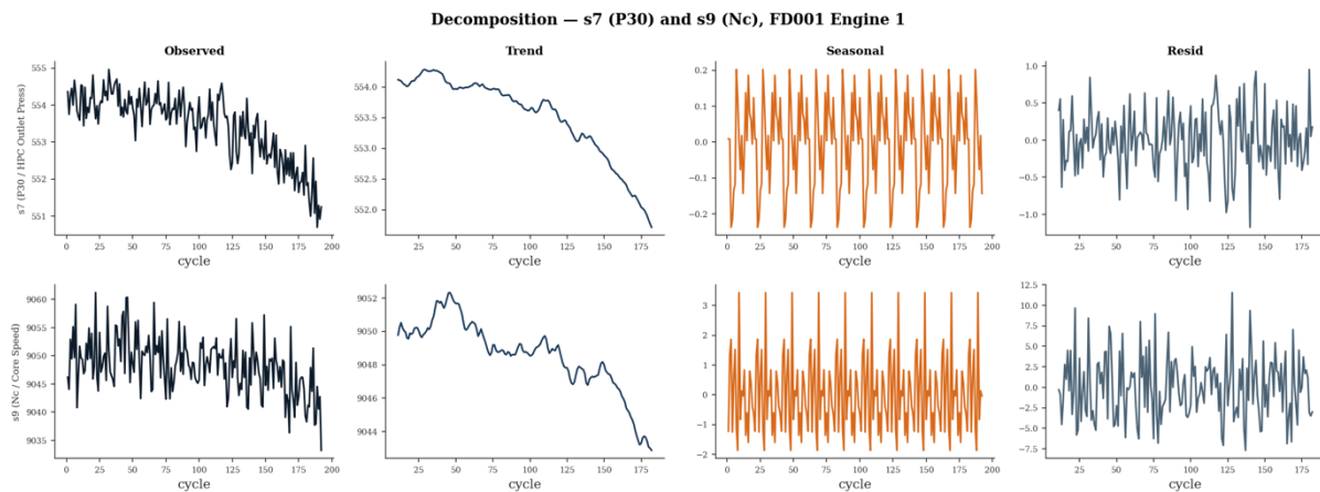
Figure 7 — STL Decomposition of Sensors s7 and s9
