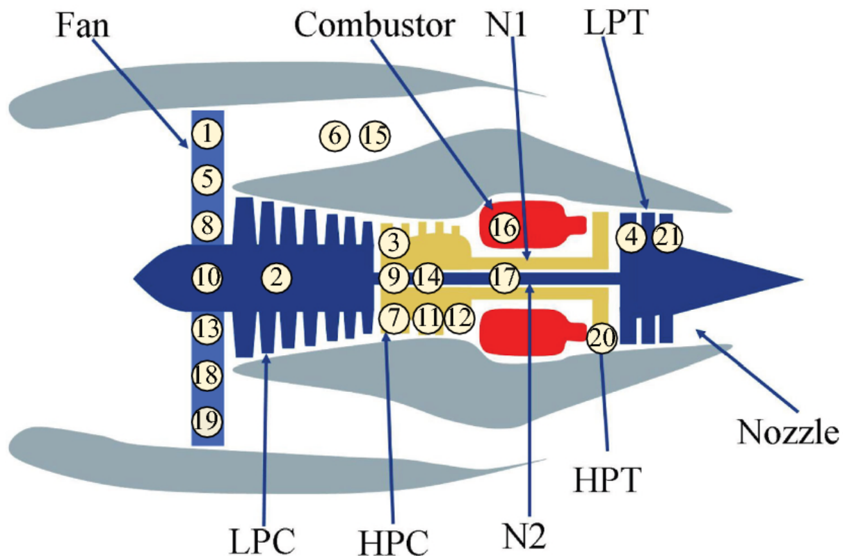
Figure 17 — C-MAPSS Turbofan Sensor Placement Diagram
