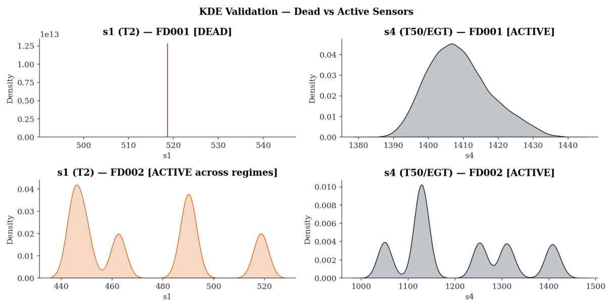
Figure 4 — Direct Comparison: Dead Sensor s1 vs Active Sensor s4
