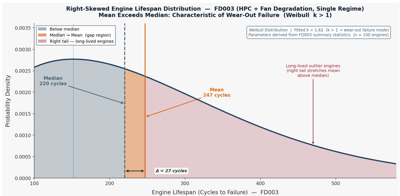
Figure 1 — RUL Distribution: 27-Cycle Gap Between Mean and Median Lifespan
