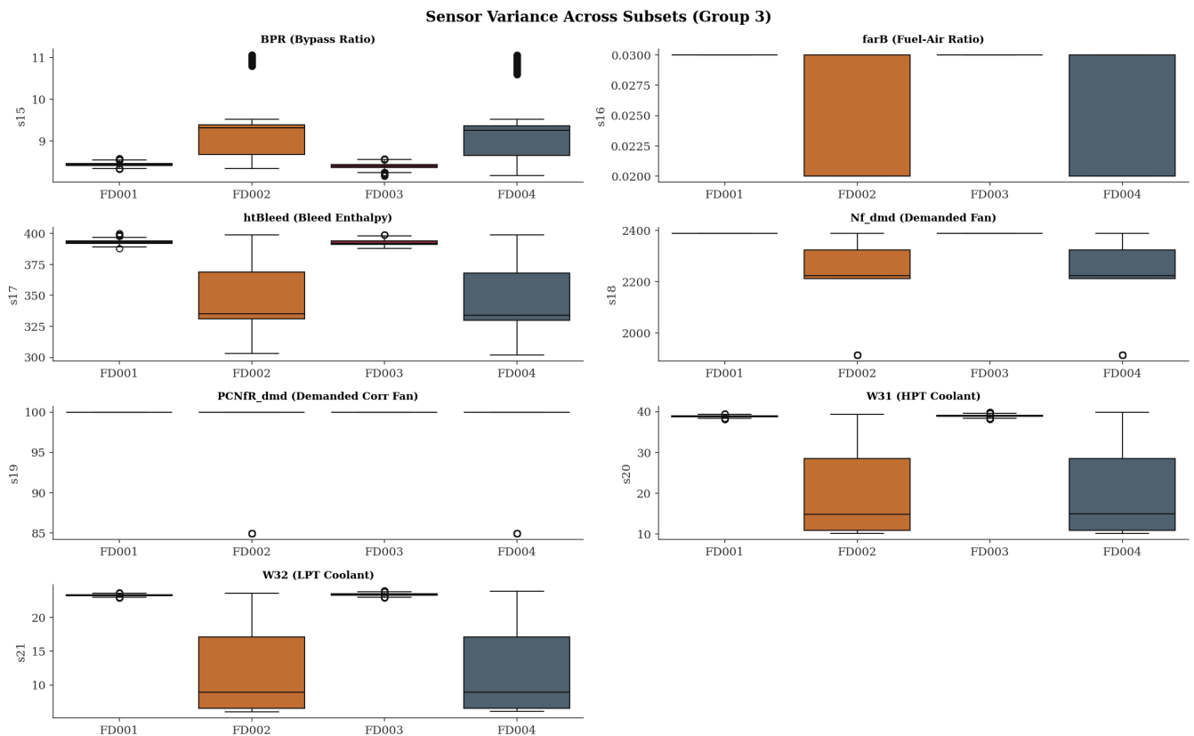
Figure 16 — Sensor Variance Across FD00x: Group 3
