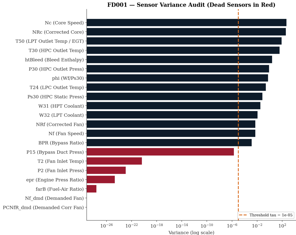
Figure 2 — Dead Sensors and Highest-Variance Active Sensor by Variance Magnitude
