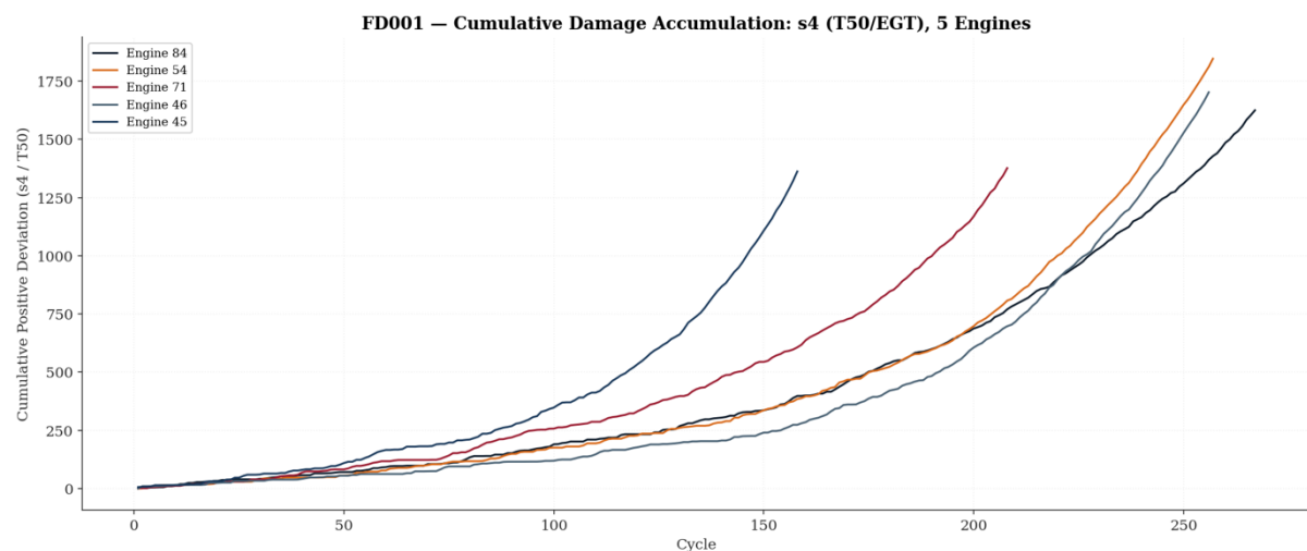
Figure 12 — Cumulative Damage Accumulation on Sensor s4 (5 Randomly Chosen Engines)
