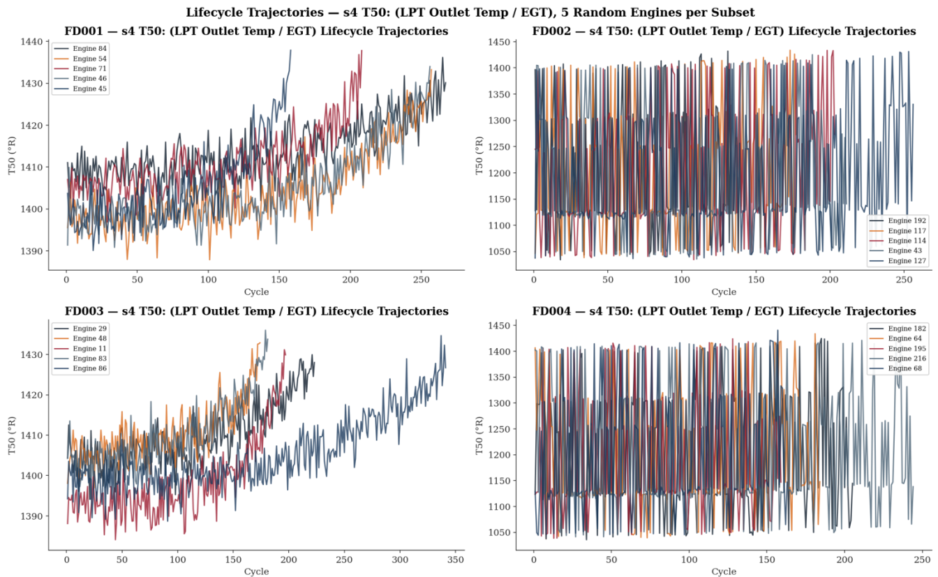
Figure 9 — Lifecycle Trajectories on Sensor s4 Across All Subsets (5 Engines)
